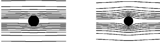
FIG. 1. Field lines of the Kaluza-Klein magnetic field \mathcal{F} for the exact solution (4.5), for the black holes that result from compactification of non-extremal and extremal strings. The radius in Eq. (4.5) has been changed to “Schwarzschild radius” r \rightarrow r - q .
