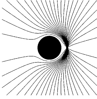
FIG. 2. Field lines of the magnetic field \mathcal{F} for the exact configuration (5.18). The radius in Eq. (5.18) has been changed to “Schwarzschild radius” r \rightarrow r - q . The “origin” of the covariantly constant field has been put at l = q/2 .
